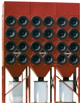
RP8-3 Dust collector, 24 cartridge
